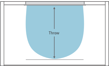
Figure 28: Continuous grille
