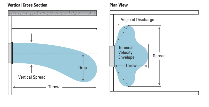
Figure 5: Drop (left), spread (right)
