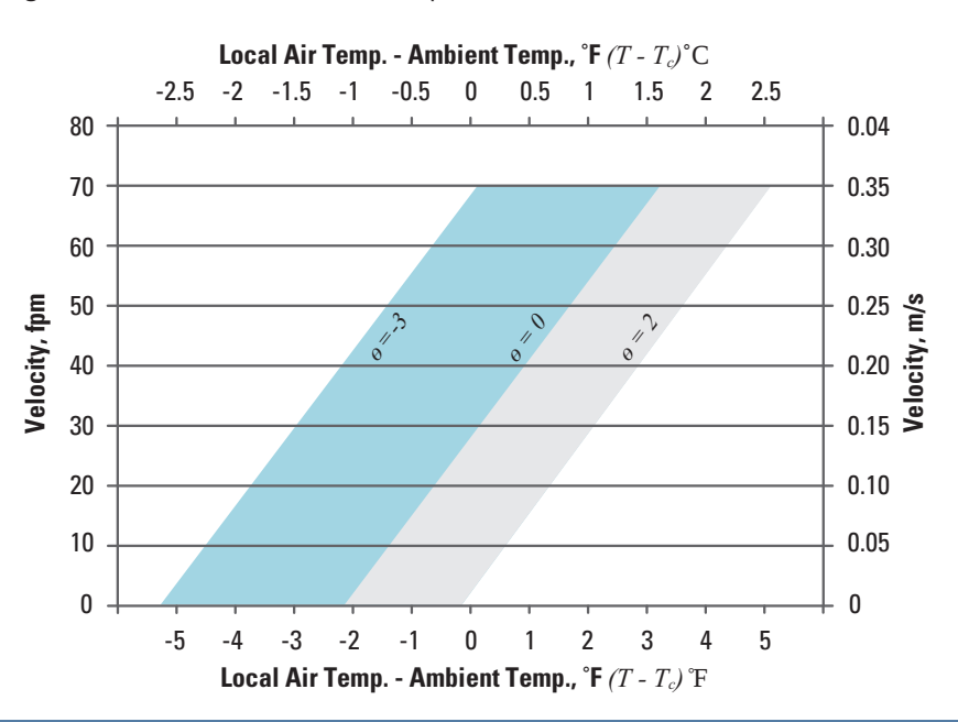
Figure 30: Comfort criteria - draft temperature
