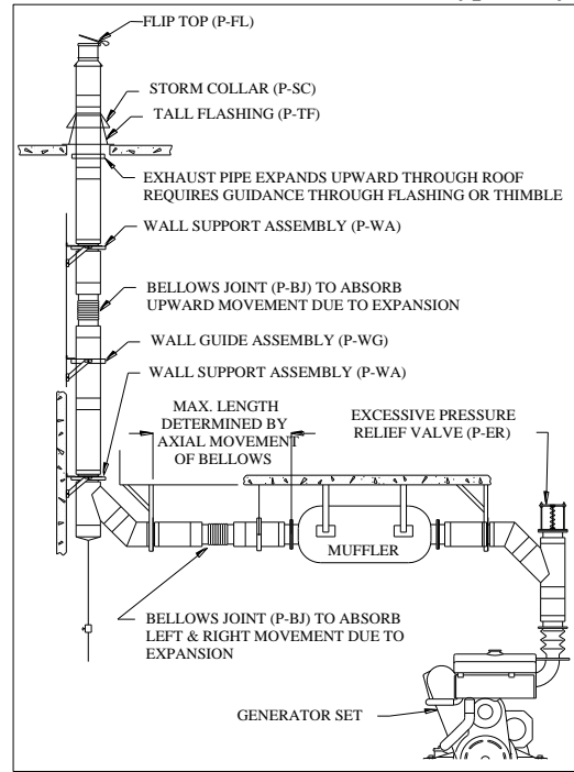
Fig. C-2 - Bellows Joints (P-BJ)
