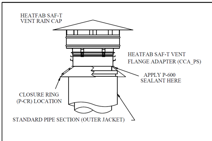
Fig. I-3 – Category II Application Termination
