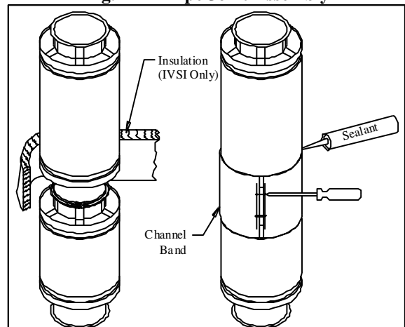
Fig. A-2 – Pipe Joint Assembly
